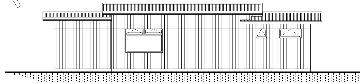
Elevation 0 - 3 scale 1:100
