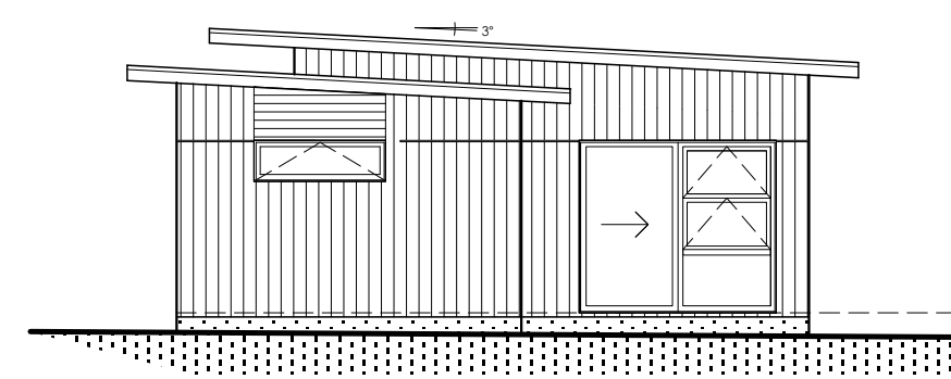
Elevation 0 - 4 scale 1:100
