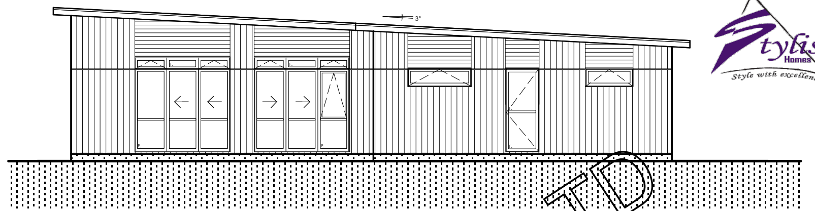
Elevation 0 - 1 scale 1:100
