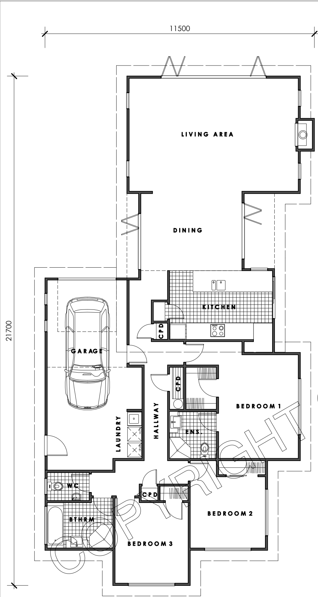
Reference Floorplan scale 1:100 Floor area = 177m 2
