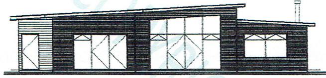
ELEVATION .3.
