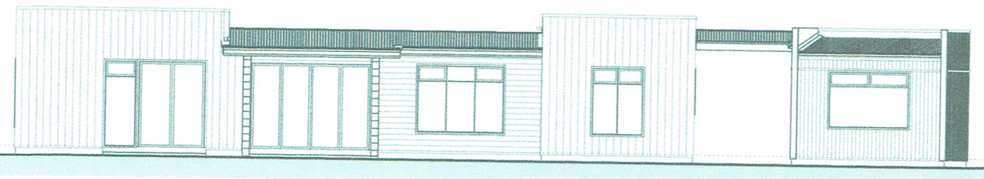
Elevation 01 Scale 1:100
