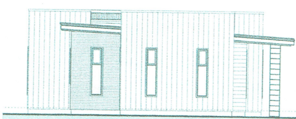
Elevation 04 Scale 1:100
