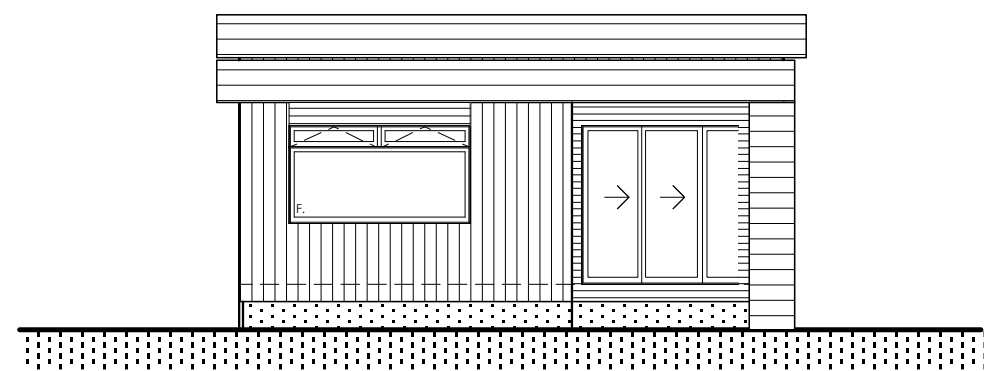
Elevation 0 - 4 scale 1:100
